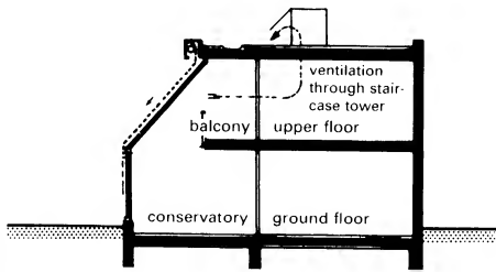
6 Section → 4 + 5
